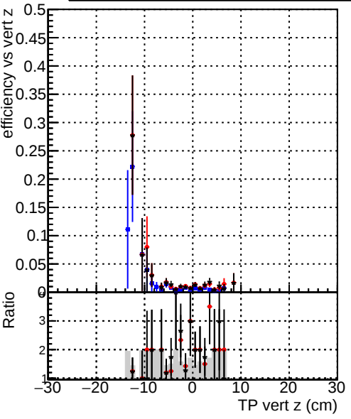
Efficiency vs TP vert z (cm) Legend: DQM_original_step2_ttbar-phase1-newgeom DQM_mkFit_step2_ttbar-phase1-newgeom DQM_pixelCPETemplate_step2_ttbar-phase1-newgeom
