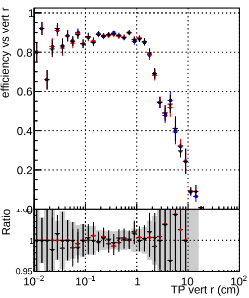
Efficiency vs TP vert r (cm) DQM_original_step2_ttbbar-phase1-newgeom DQM_mkFit_step2_ttbbar-phase1-newgeom DQM_pixelCPETemplate_step2_ttbbar-phase1-newgeom
