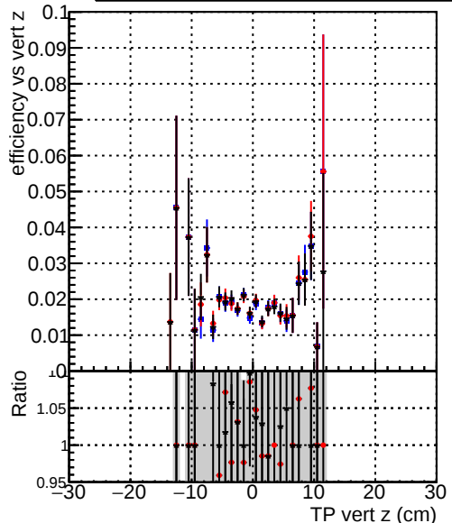
Efficiency vs. sim PV z —●— DQM_original_step2_ttbar-phase1-newgeom —●— DQM_mkFit_step2_ttbar-phase1-newgeom —●— DQM_pixelCPETemplate_step2_ttbar-phase1-newgeom
