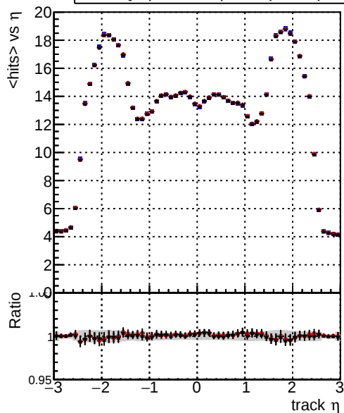
mean hits — DQM_original_step2_ttbbar-phase1-newgeom — DQM_mkFit_step2_ttbbar-phase1-newgeom — DQM_pixelCPETemplate_step2_ttbbar-phase1-newgeom
