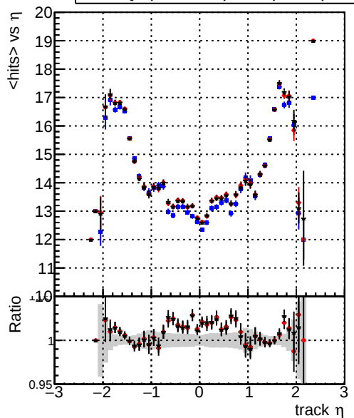
mean hits vs \eta — DQM_original_step2_ttbar-phase1-newgeom — DQM_mkFit_step2_ttbar-phase1-newgeom — DQM_pixelCPETemplate_step2_ttbar-phase1-newgeom
