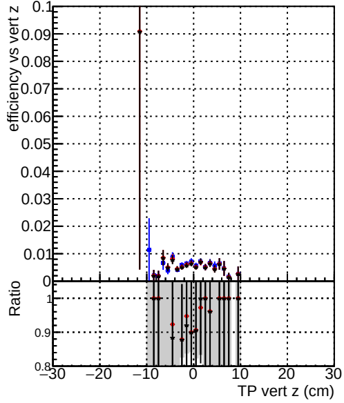
Efficiency vs. sim PV z —•— DQM_original_step2_ttbbar-phase1-newgeom —•— DQM_mkFit_step2_ttbbar-phase1-newgeom —•— DQM_pixelCPETemplate_step2_ttbbar-phase1-newgeom
