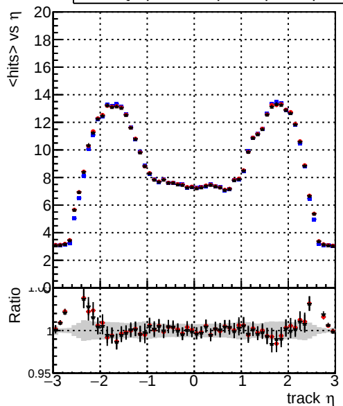
mean hits — DQM_original_step2_ttbbar-phase1-newgeom — DQM_mkFit_step2_ttbbar-phase1-newgeom — DQM_pixelCPETemplate_step2_ttbbar-phase1-newgeom
