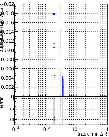
Legend: DQM_original_step2_ttbar-phase1-newgeom (blue squares), DQM_mkFit_step2_ttbar-phase1-newgeom (red circles), DQM_pixelCPETemplate_step2_ttbar-phase1-newgeom (black crosses)
