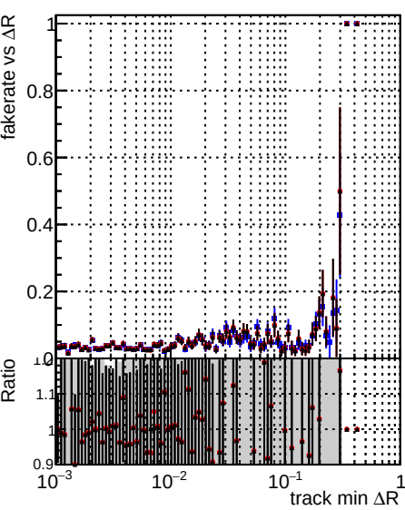
Legend: - blue line with dots: DQM_original_step2_pt200_eta2p0to2p5 - red line with dots: DQM_mkFit_step2_pt200_eta2p0to2p5 - black line with dots: DQM_pixelCPETemplate_step2_pt200_eta2p0to2p5
