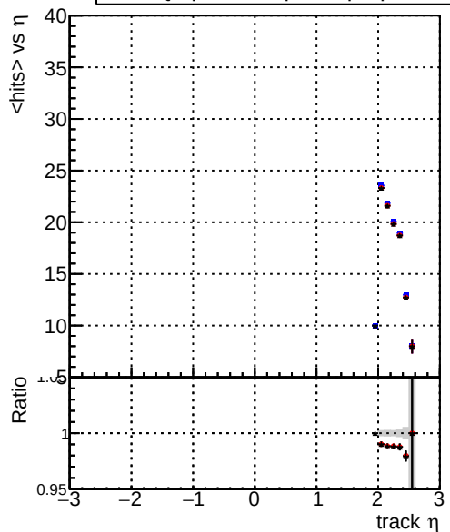
mean hits vs \eta — DQM_original_step2_pt200_eta2p0to2p5 — DQM_mkFit_step2_pt200_eta2p0to2p5 — DQM_pixelCPEtemplate_step2_pt200_eta2p0to2p5
