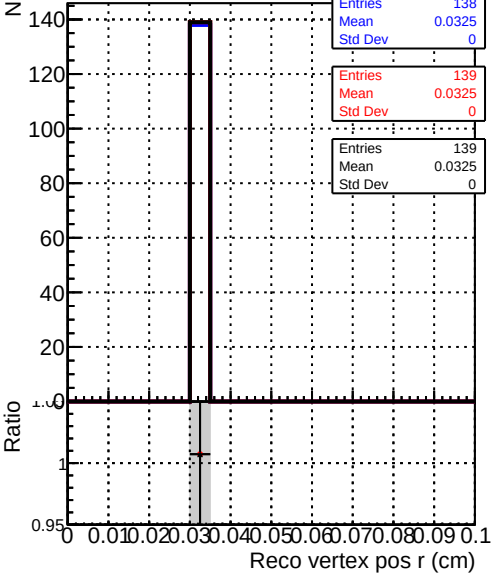
Recons Legend: DQM_original_step2_pt200_eta2p0to2p5 (blue) DQM_mkFit_step2_pt200_eta2p0to2p5 (red) DQM_pixelCPETemplate_step2_pt200_eta2p0to2p5 (black)
