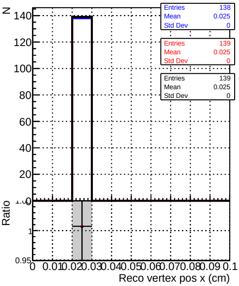
Recons Legend: DQM_original_step2_pt200_eta2p0to2p5 (blue) DQM_mkFit_step2_pt200_eta2p0to2p5 (red) DQM_pixelCPETemplate_step2_pt200_eta2p0to2p5 (black)
