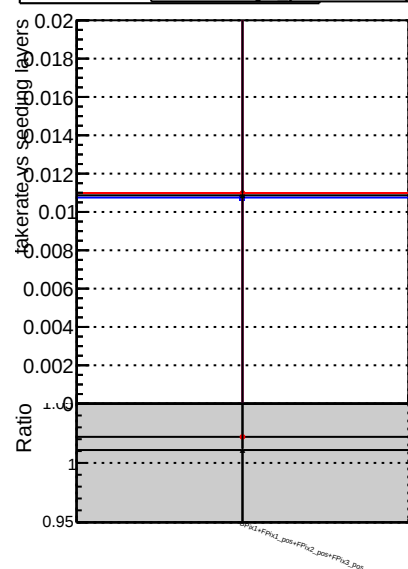
Fake rate vs. DOM original step2 pt200 eta2p0to2p5 DOM mkr-it step2 pt200 eta2p0to2p5 DOM pixelCPE template step2 pt200 eta2p0to2p5
