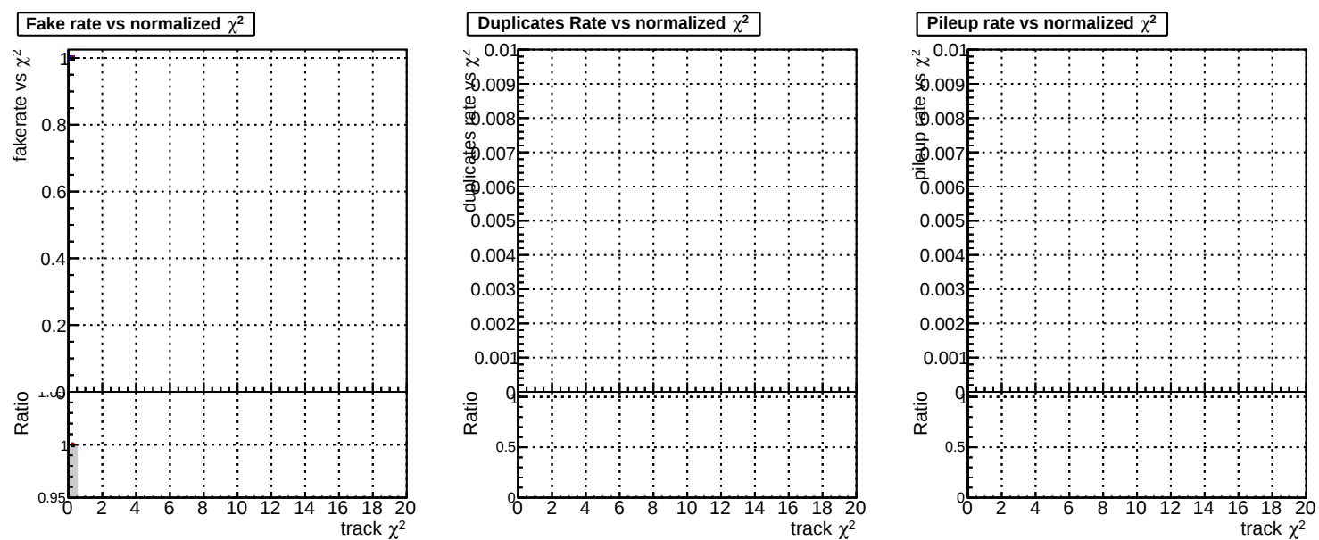
Fake rate vs. DOM original step2 pt200 eta2p0to2p5 DOM mkr-it step2 pt200 eta2p0to2p5 DOM pixelCPE template step2 pt200 eta2p0to2p5
