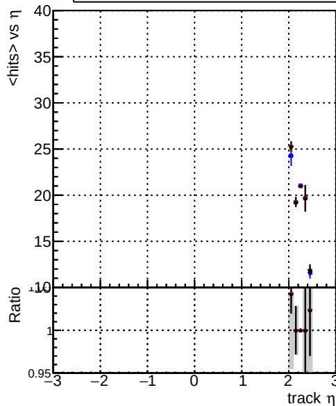
mean hits — DQM_original_step2_pt200_eta2p0to2p5 — DQM_mkFit_step2_pt200_eta2p0to2p5 — DQM_pixelCPEtemplate_step2_pt200_eta2p0to2p5
