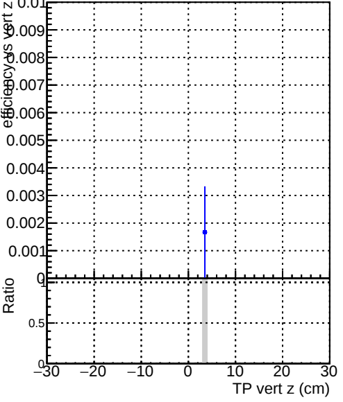
Efficiency vs vert z Legend: DQM_original_step2_pt200_eta2p0to2p5 DQM_mkFit_step2_pt200_eta2p0to2p5 DQM_pixelCPETemplate_step2_pt200_eta2p0to2p5
