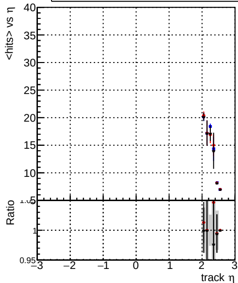
mean hit — DQM_original_step2_pt200_eta2p0to2p5 — DQM_mkFit_step2_pt200_eta2p0to2p5 — DQM_pixelCPETemplate_step2_pt200_eta2p0to2p5
