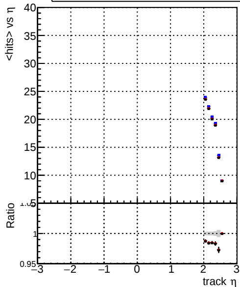
mean hits vs \eta — DQM_original_step2_pt200_eta2p0to2p5 — DQM_mkFit_step2_pt200_eta2p0to2p5 — DQM_pixelCPETemplate_step2_pt200_eta2p0to2p5
