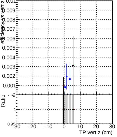
Efficiency vs vert z Legend: DQM_original_step2_pt200_eta2p0to2p5 (blue circles) DQM_mkFit_step2_pt200_eta2p0to2p5 (red circles) DQM_pixelCPETemplate_step2_pt200_eta2p0to2p5 (black circles)
