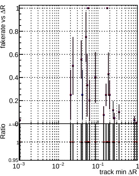
Fake rate vs \Delta R(\text{track, jet}) DQM_original_step2_pt1to20_eta2p5to4p0 DQM_mkFit_step2_pt1to20_eta2p5to4p0 DQM_pixelCPETemplate_step2_pt1to20_eta2p5to4p0
