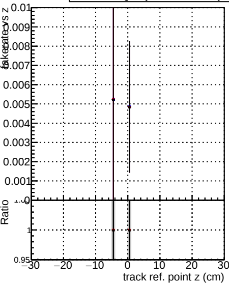
Fake rate vs verpos DQM_original_step2_pt1to20_eta2p5to4p0 DQM_mkFit_step2_pt1to20_eta2p5to4p0 DQM_pixelCPETemplate_step2_pt1to20_eta2p5to4p0
