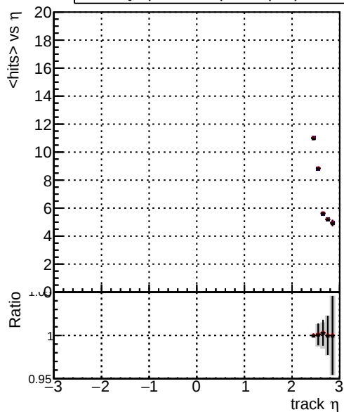
mean hits — DQM_original_step2_pt1to20_eta2p5to4p0 — DQM_mkFit_step2_pt1to20_eta2p5to4p0 — DQM_pixelCPETemplate_step2_pt1to20_eta2p5to4p0
