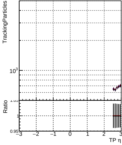
N of simulated tracks vs \eta Legend: DQM_original_step2_pt1to20_eta2p5to4p0 DQM_mkFit_step2_pt1to20_eta2p5to4p0 DQM_pixelCPETemplate_step2_pt1to20_eta2p5to4p0
