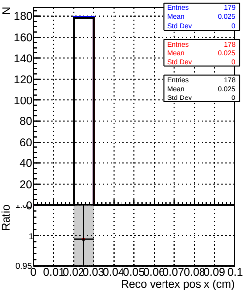
ReconstructedAllAssoc2Gen_X
