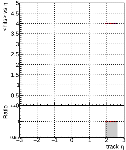
— DQM_original_step2_pt1to20_eta2p0to2p5 — DQM_mkFit_step2_pt1to20_eta2p0to2p5 — DQM_pixelCPETemplate_step2_pt1to20_eta2p0to2p5
