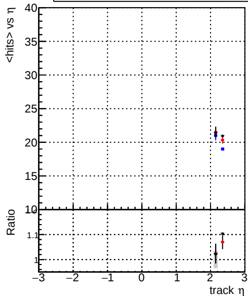
mean hits vs \eta — DQM_original_step2_pt1to20_eta2p0to2p5 — DQM_mkFit_step2_pt1to20_eta2p0to2p5 — DQM_pixelCPEtemplate_step2_pt1to20_eta2p0to2p5
