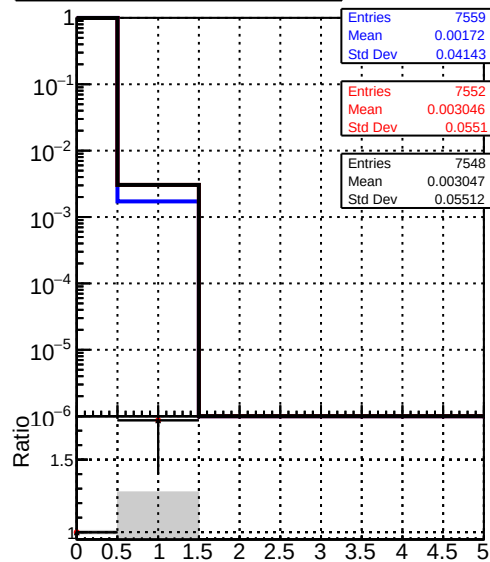
mean hit — DQM_original_step2_pt1to20_eta2p0to2p5 — DQM_mkFit_step2_pt1to20_eta2p0to2p5 — DQM_pixelCPEtemplate_step2_pt1to20_eta2p0to2p5
