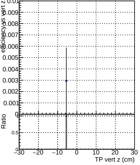
Efficiency vs vert z Legend: DQM_original_step2_pt1to20_eta2p0to2p5 DQM_mkFit_step2_pt1to20_eta2p0to2p5 DQM_pixelCPETemplate_step2_pt1to20_eta2p0to2p5
