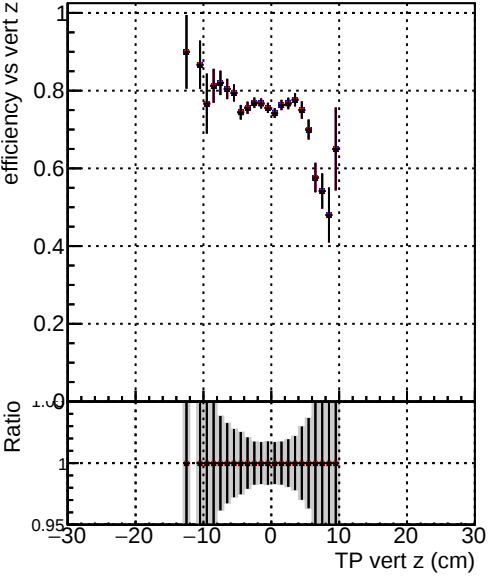
Efficiency vs Sim. PV z Legend: DQM_original_step2_pt1to20_eta2p0to2p5 DQM_mkFit_step2_pt1to20_eta2p0to2p5 DQM_pixelCPETemplate_step2_pt1to20_eta2p0to2p5
