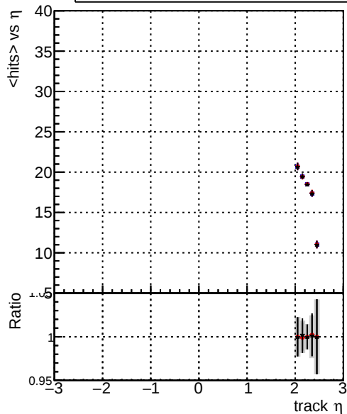
mean hit — DQM_original_step2_pt1to20_eta2p0to2p5 — DQM_mkFit_step2_pt1to20_eta2p0to2p5 — DQM_pixelCPEtemplate_step2_pt1to20_eta2p0to2p5
