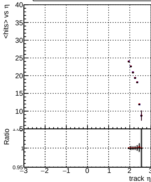
mean hits — DQM_original_step2_pt1to20_eta2p0to2p5 — DQM_mkFit_step2_pt1to20_eta2p0to2p5 — DQM_pixelCPEtemplate_step2_pt1to20_eta2p0to2p5
