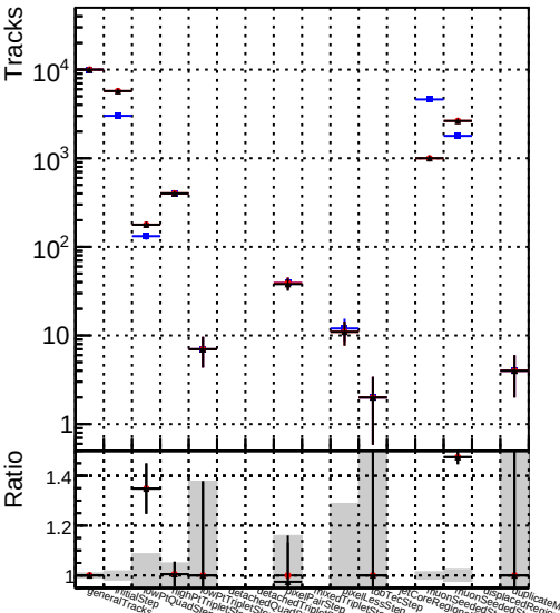
Number DQM_original_step2_pt1to20_eta1p6to2p0 DQM_mkFit_step2_pt1to20_eta1p6to2p0 DQM_pixelCPETemplate_step2_pt1to20_eta1p6to2p0
