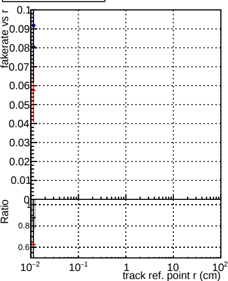
Fake rate vs v —•— DQM_original_step2_pt1to20_eta1p6to2p0 —•— DQM_mkFit_step2_pt1to20_eta1p6to2p0 —•— DQM_pixelCPETemplate_step2_pt1to20_eta1p6to2p0
