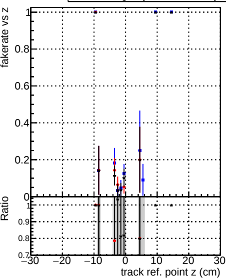
Fake rate vs v —•— DQM_original_step2_pt1to20_eta1p6to2p0 —•— DQM_mkFit_step2_pt1to20_eta1p6to2p0 —•— DQM_pixelCPETemplate_step2_pt1to20_eta1p6to2p0
