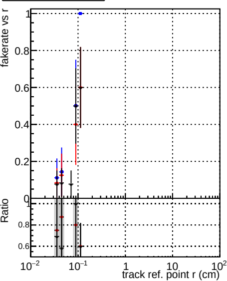
Fake rate vs vertpos — DQM_original_step2_pt1to20_eta1p6to2p0 — DQM_mkFit_step2_pt1to20_eta1p6to2p0 — DQM_pixelCPETemplate_step2_pt1to20_eta1p6to2p0
