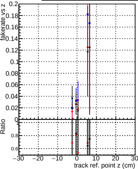
Fake rate vs vertpos — DQM_original_step2_pt1to20_eta1p6to2p0 — DQM_mkFit_step2_pt1to20_eta1p6to2p0 — DQM_pixelCPETemplate_step2_pt1to20_eta1p6to2p0
