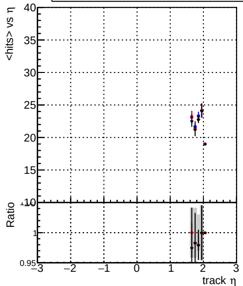
mean hit — DQM_original_step2_pt1to20_eta1p6to2p0 — DQM_mkFit_step2_pt1to20_eta1p6to2p0 — DQM_pixelCPEtemplate_step2_pt1to20_eta1p6to2p0
