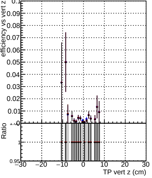
Efficiency vs TP vert z (cm) plot Legend: DQM_original_step2_pt1to20_eta1p6to2p0 DQM_mkFit_step2_pt1to20_eta1p6to2p0 DQM_pixelCPETemplate_step2_pt1to20_eta1p6to2p0
