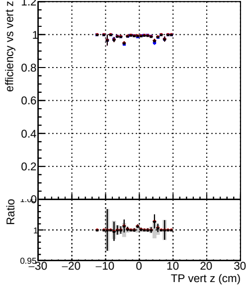
Efficiency vs. TP vert z (cm) Legend: DQM_original_step2_pt1to20_eta1p6to2p0 DQM_mkFit_step2_pt1to20_eta1p6to2p0 DQM_pixelCPETemplate_step2_pt1to20_eta1p6to2p0
