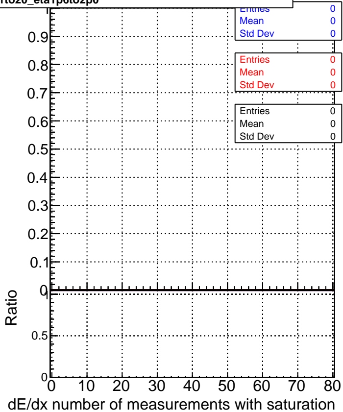
■ DQM_original_step2_pt1to20_eta1p6to2p0 ● DQM_mkFit_step2_pt1to20_eta1p6to2p0 ▲ DQM_pixelCPETemplate_step2_pt1to20_eta1p6to2p0
