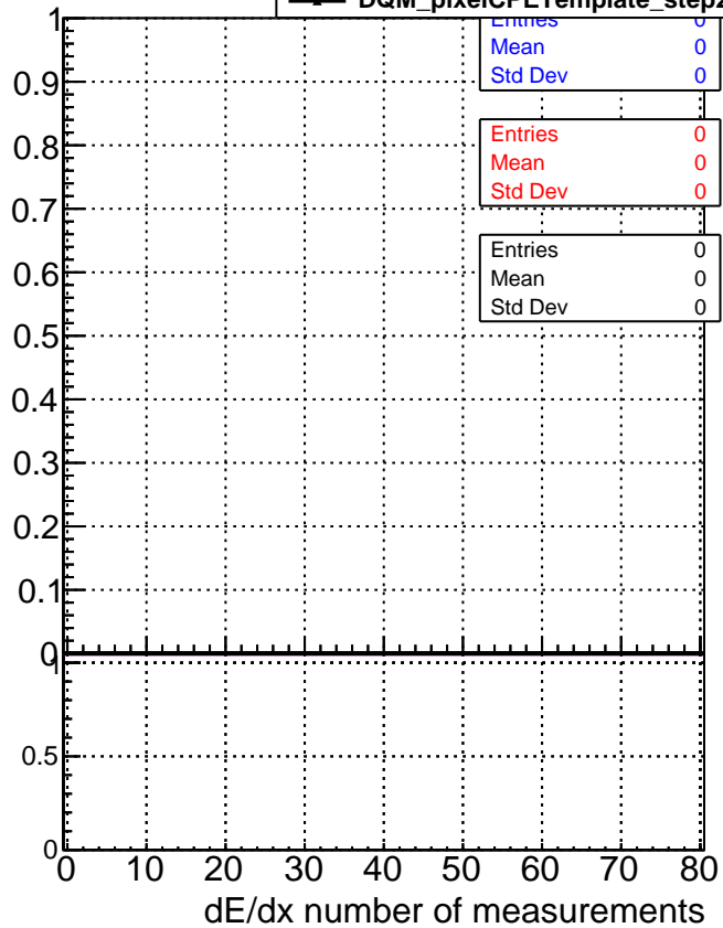
■ DQM_original_step2_pt1to20_eta1p6to2p0 ● DQM_mkFit_step2_pt1to20_eta1p6to2p0 ▲ DQM_pixelCPETemplate_step2_pt1to20_eta1p6to2p0
