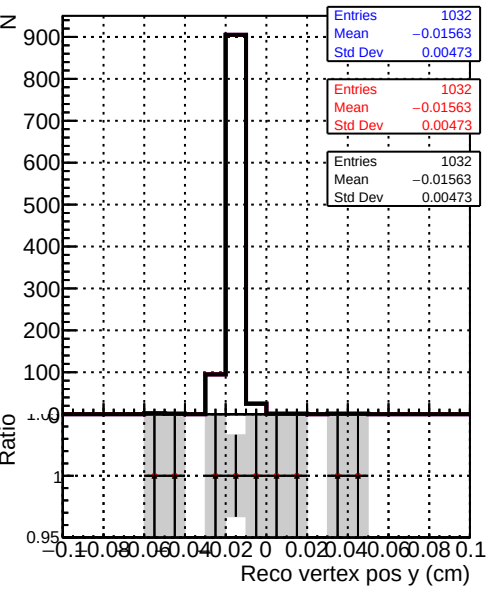
Recons Legend: DQM_original_step2_pt1to20_eta1p6to2p0 (blue line), DQM_mkFit_step2_pt1to20_eta1p6to2p0 (red line), DQM_pixelCPETemplate_step2_pt1to20_eta1p6to2p0 (black line)
