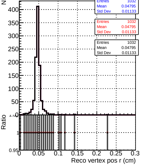
Recons Legend: DQM_original_step2_pt1to20_eta1p6to2p0 (blue line), DQM_mkFit_step2_pt1to20_eta1p6to2p0 (red line), DQM_pixelCPETemplate_step2_pt1to20_eta1p6to2p0 (black line)
