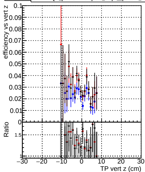
Efficiency —●— DQM_mkFit_step2_pt1to20_eta1p6to2p0 —▲— DQM_pixelCPETemplate_step2_pt1to20_eta1p6to2p0
