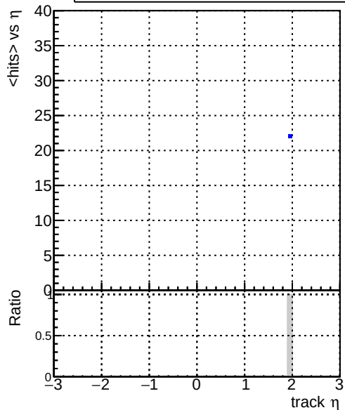
mean hits — DQM_original_step2_pt1to20_eta1p6to2p0 — DQM_mkFit_step2_pt1to20_eta1p6to2p0 — DQM_pixelCPETemplate_step2_pt1to20_eta1p6to2p0
