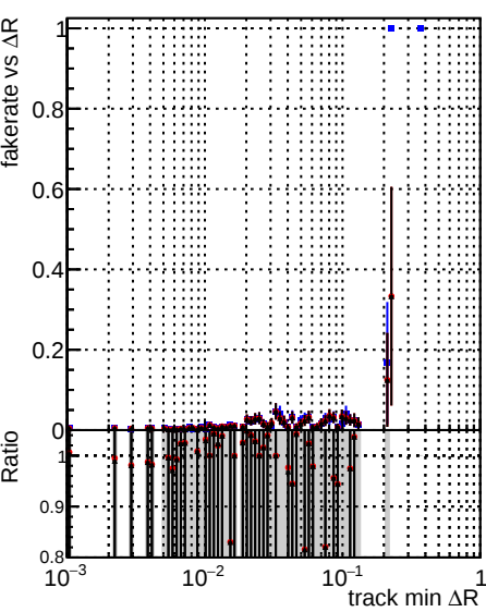
Legend: DQM_original_step2_pt1to20_eta1p4to1p6 (blue squares), DQM_mkFit_step2_pt1to20_eta1p4to1p6 (red circles), DQM_pixelCPETemplate_step2_pt1to20_eta1p4to1p6 (black crosses)
