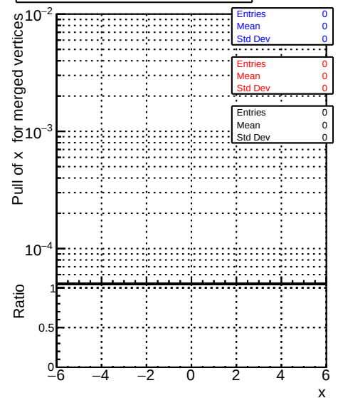
RecoAllAssoc2GenMatchedMerged_PullX
