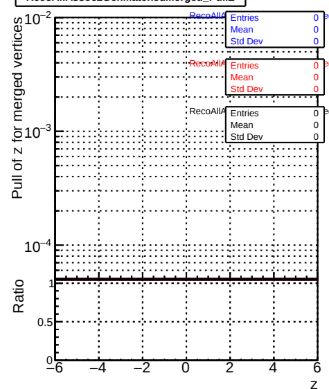
RecoAllAssoc2GenMatchedMerged_PullZ
