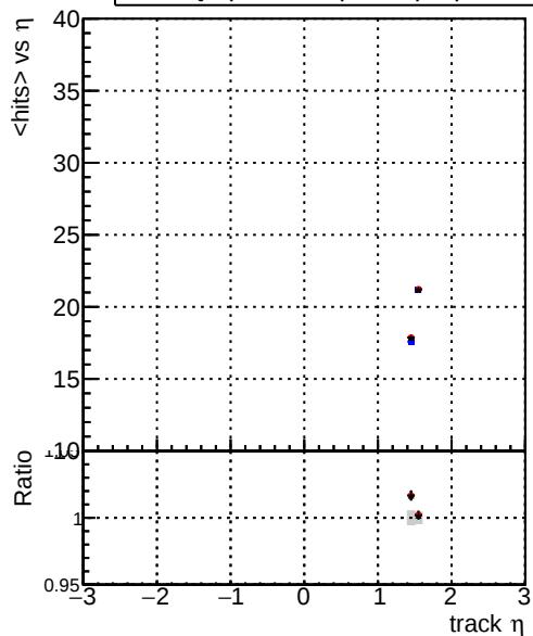
mean hits — DQM_original_step2_pt1to20_eta1p4to1p6 — DQM_mkFit_step2_pt1to20_eta1p4to1p6 — DQM_pixelCPETemplate_step2_pt1to20_eta1p4to1p6
