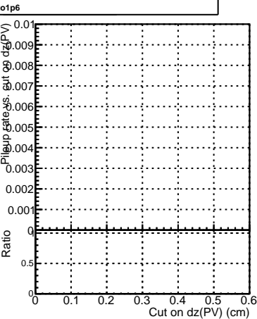
Pileup rate
