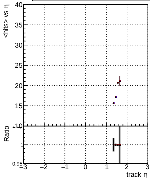
mean hits vs \eta DQM_original_step2_pt1to20_eta1p4to1p6 DQM_mkFit_step2_pt1to20_eta1p4to1p6 DQM_pixelCPETemplate_step2_pt1to20_eta1p4to1p6
