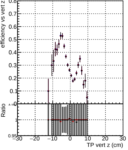
Efficiency vs Sim. PV z Legend: DQM_original_step2_pt1to20_eta1p4to1p6 DQM_mkFit_step2_pt1to20_eta1p4to1p6 DQM_pixelCPETemplate_step2_pt1to20_eta1p4to1p6
