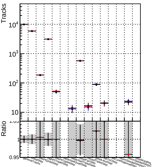
Number DQM_original_step2_pt1to20_eta1p0to1p4 DQM_mkFit_step2_pt1to20_eta1p0to1p4 DQM_pixelCPETemplate_step2_pt1to20_eta1p0to1p4
