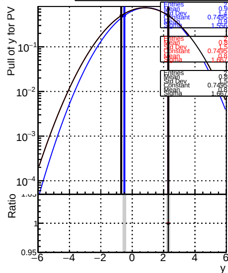
RecoPVAssoc Legend: DQM original step2_pt1to20_eta1p0to1p4 DQM mkFit step2_pt1to20_eta1p0to1p4 DQM_pixelCPETemplate step2_pt1to20_eta1p0to1p4
