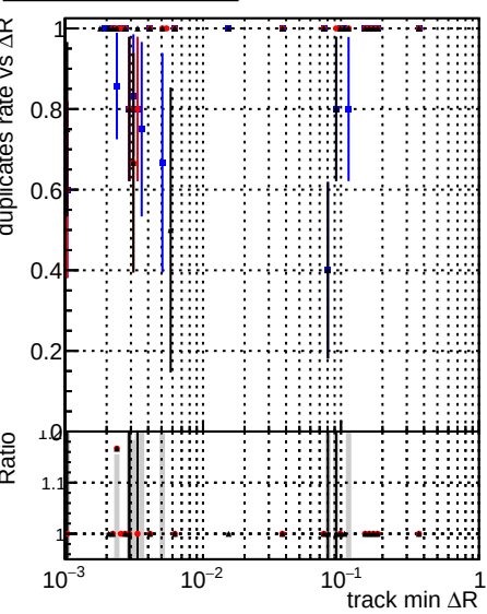
Legend: DQM original step2 pt1to20 eta1p0to1p4 (blue), DQM mkFit step2 pt1to20 eta1p0to1p4 (red), DQM pixelCPE template step2 pt1to20 eta1p0to1p4 (black)
