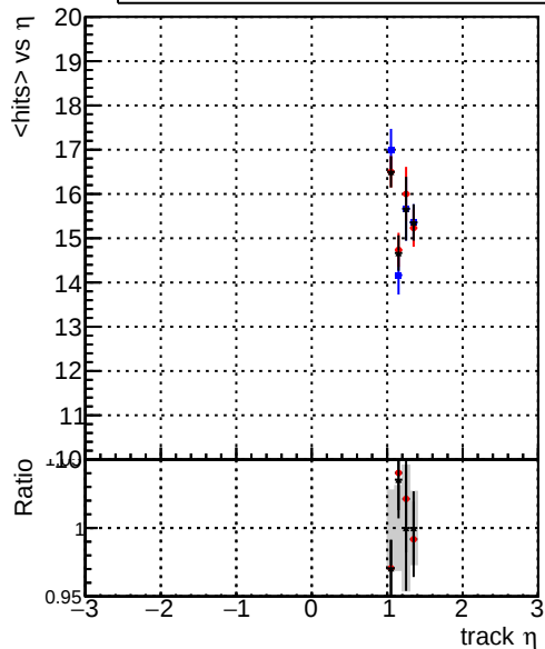
— DQM_original_step2_pt1to20_eta1p0to1p4 — DQM_mkFit_step2_pt1to20_eta1p0to1p4 — DQM_pixelCPEtemplate_step2_pt1to20_eta1p0to1p4 mean hits
