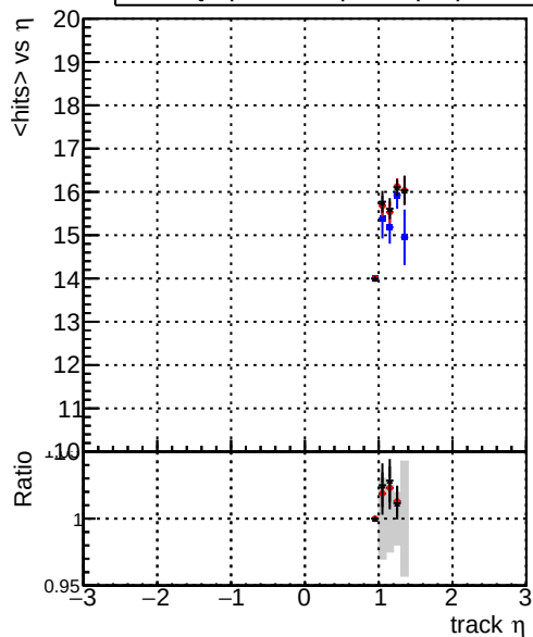
mean hits vs \eta — DQM_original_step2_pt1to20_eta1p0to1p4 — DQM_mkFit_step2_pt1to20_eta1p0to1p4 — DQM_pixelCPEtemplate_step2_pt1to20_eta1p0to1p4
